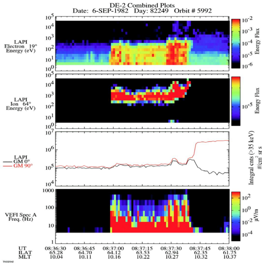
Figure 4. DE-2 data from September, 6, 1982. Data was taken during an equatorward cusp pass in the southern hemisphere. The top spectrogram is electrons measured at a 19( pitch angle. The second is ions measured at a pitch angle of 64(. The third plot contains high energy electrons integrated for energies greater than 35 keV and 0( and 90( pitch angle, and the bottom spectrogram is measured square root of the electric wave power.
