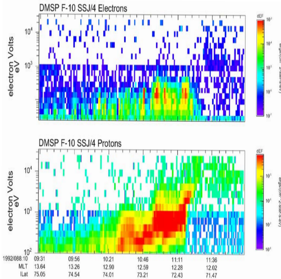
Figure 6. DMSP F-10 data from March 28, 1992. Data was taken during an equatorward cusp pass in the northern hemisphere. Upper spectrogram is electrons, and the lower spectrogram is ions.
