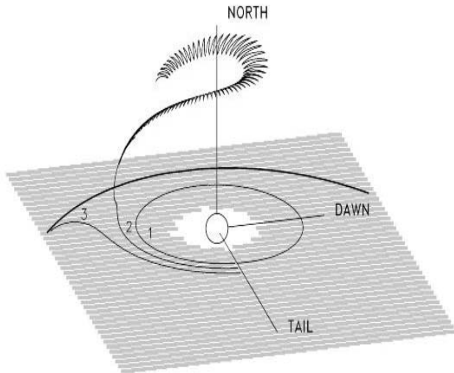
Figure 17. Equatorial ring current particles drift from the plasma sheet to the dayside magnetopause region and are deflected into a cusp-orbiting trajectory. From here they may be lost along the edges of the cusp to low altitudes. (from Delcourt and Sauvaud,1999)
