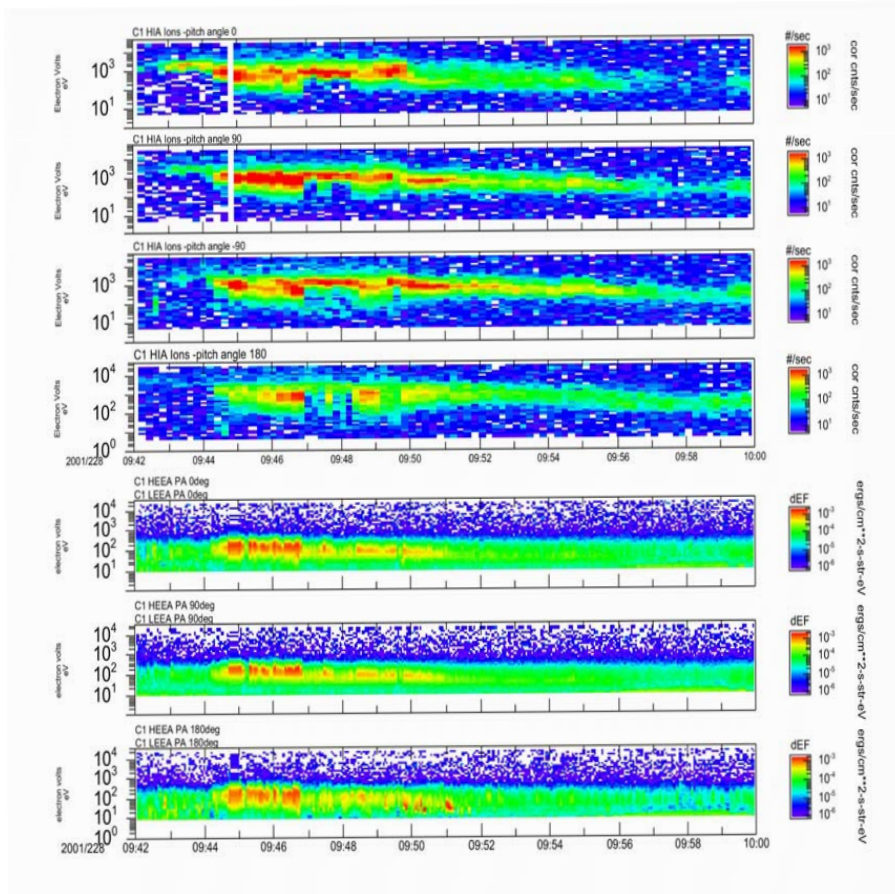
Figure 13. Cluster-1 data from August, 16, 2001. Top four panels are HIA ions for in the parallel, perpendicular, and antiparallel directions. Bottom three panels are PEACE electrons for the same pitch angle directions.
