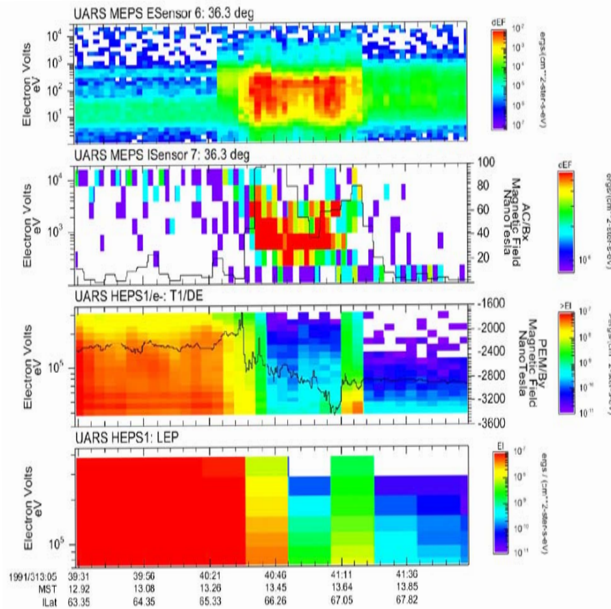
Figure 10. UARS data from November, 9, 1991. The top two spectrograms are medium energy electrons and ions, while the lower two are high energy electrons and ions. The upper line plot is the integrated square root of magnetic wave power, while the lower line plot is magnetic field perpendicular to the spacecraft.
