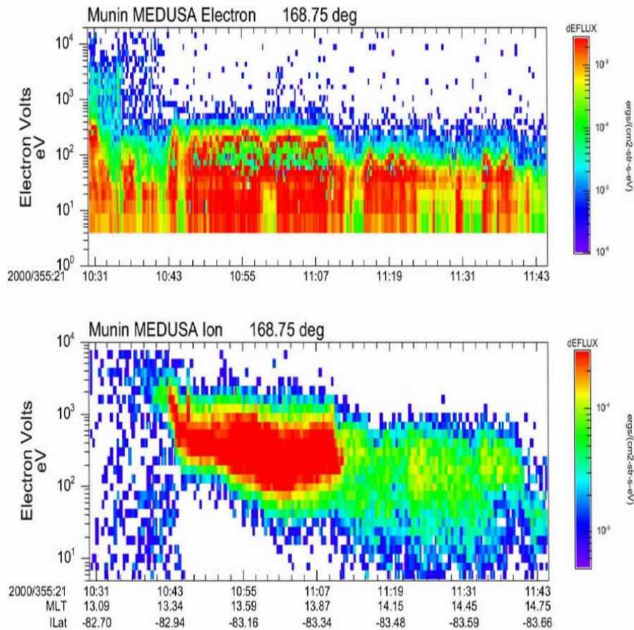
Figure 9. Munin data from December, 20, 2000. Data from a poleward cusp pass in the southern hemisphere. The upper spectrogram is precipitating electrons, and the lower spectrogram shows the ions for the same look direction. A very small V feature can be seen at the equatorward (left) edge of the ion flux in the lower panel, near 21:10:43 UT.
