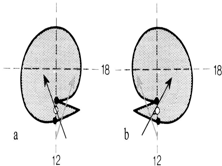
Figure 15. Diagram showing possible cusp wedge traversals in high B_y cases. The Sun is towards the bottom of the figure marked by a 12. (a) The northern polar cap for duskward IMF (or southern polar cap for dawnward IMF). (b) The northern polar cap for dawnward IMF (or southern polar cap for duskward IMF). In each case, a satellite track represented by the gray arrow would see a V structure, while a satellite track marked as black, would not. (adapted from Crooker, 1988).
