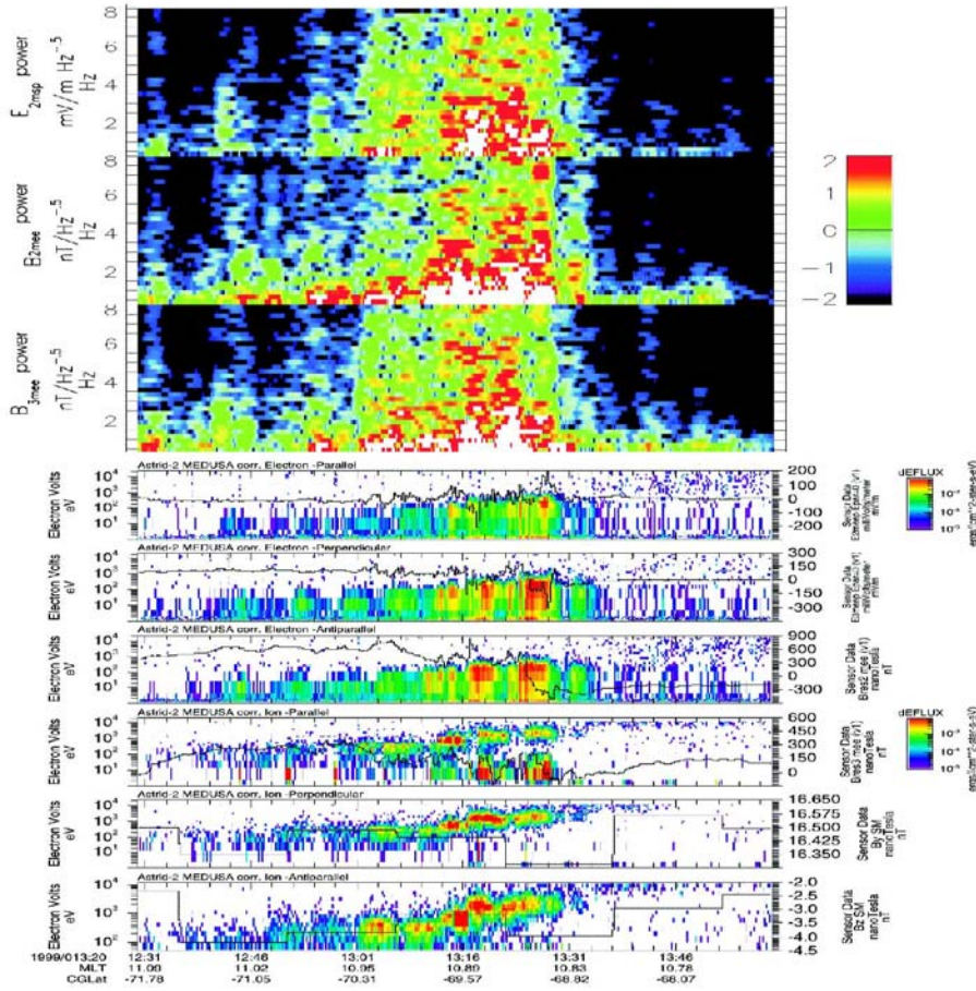
Figure 8. Astrid-2 data from January, 13, 1999. The data are taken during an equatorward pass through the southern cusp region. The top three panels contain frequency-time spectrograms of electric (top) and magnetic (second two) waves. The middle three panels contain electron fluxes and the bottom three panels ion fluxes. For both the electrons and ions, the top panel contains particles at "zero" pitch angle (flowing up the field line). The middle particle panels are trapped particles (90( pitch angle) and the bottom set contain downcoming particles (180( pitch angle). The fourth and fifth panels also contain line plots of the two perpendicular electric field components (with a scale on the right). Panels six and seven display residual magnetic field intensity (after subtracting a model field) for the same two perpendicular directions as the electric field. The bottom two line plots are the y and z components of the IMF as measured by IMP-8.
