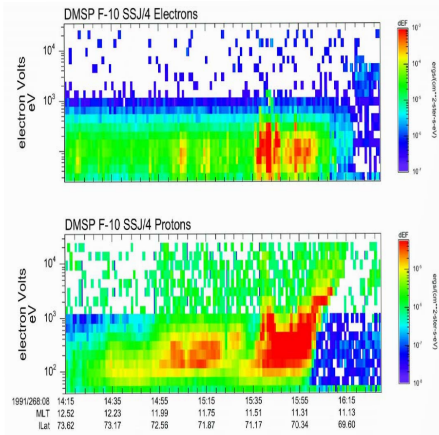
Figure 7. DMSP F-10 data from September 25, 1991. Data was taken during an equatorward cusp pass in the northern hemisphere. Upper spectrogram is electrons, and the lower spectrogram is ions.
