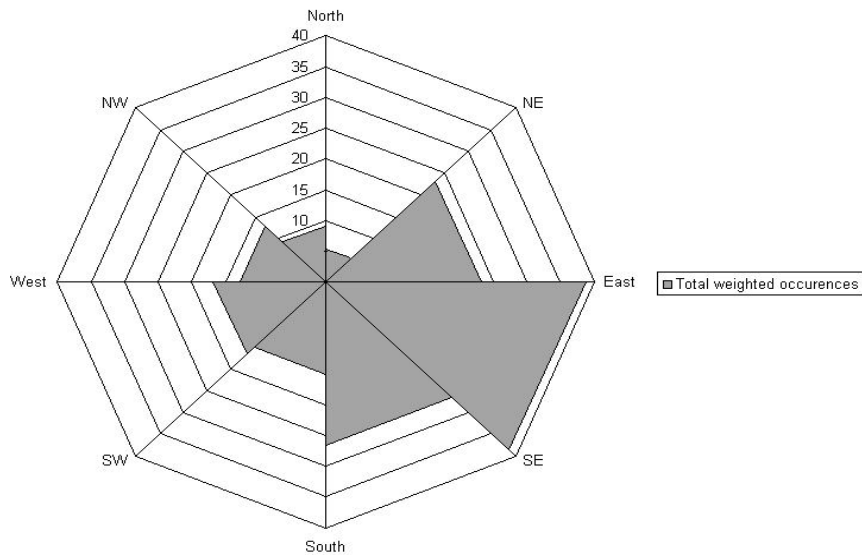
Figure 16. Histogram of weighted "V" Occurrences vs. IMF clock angle. A strong duskward and weaker dawnward peak can be seen as expected.
