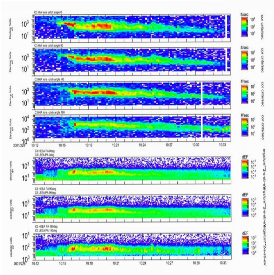
Figure 14. Cluster-3 data from August, 16, 2001. Top four panels are HIA ions for in the parallel, perpendicular, and antiparallel directions. Bottom three panels are PEACE electrons for the same pitch angle directions.
